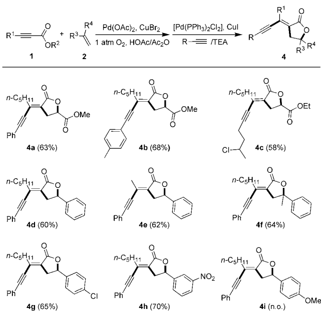
Scheme 4. Conversion of vinyl bromides to multifunctional lactones. The carboesterification reactions were carried out at 100 °C under 1 atm of O 2 with alkynoates (0.5 mmol), alkenes (0.6 mmol), Pd(OAc) 2 (5 mol %), CuBr 2 (1 mmol), and AcOH/Ac 2 O = 1:1 (v/v, 1 mL) for 12 h. The crude products were extracted with diethyl ether. Terminal alkynes (0.6 mmol), [Pd(PPh 3 ) 2 Cl 2 ] (5 mol %), CuI (5 mol %), TEA (0.1 mL), and DMF (1.5 mL) were added and the Sonogashira coupling was carried out at 80 °C for 8 h. TEA = triethylamine.
