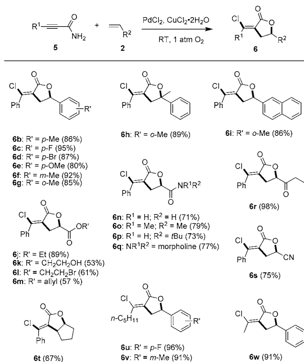
Scheme 5. Carboesterification of alkenes with alkynamides: The reactions were carried out under 1 atm of O 2 , with alkynes (0.5 mmol), alkenes (0.6 mmol), PdCl 2 (5 mol %), and CuCl 2 ·2H 2 O (1 mmol) in acetonitrile (0.5 mL) for 12 h.
